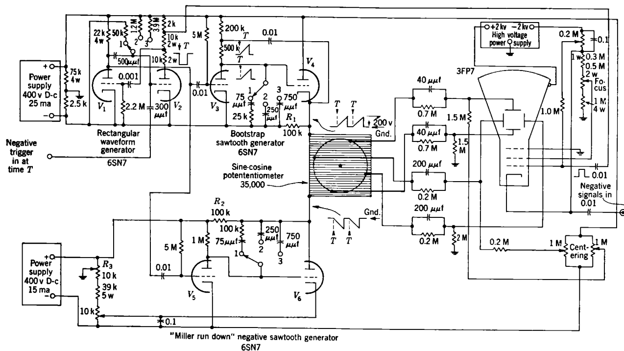
Fig. 13-11.—RTB display circuit employing a sine-cosine potentiometer and an electrostatic-deflection cathode-ray tube.
